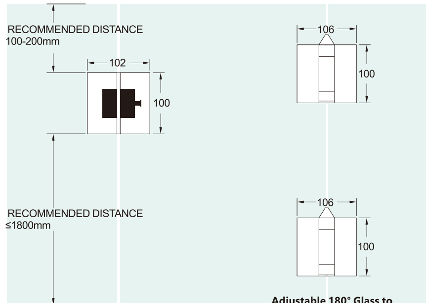
Adjustable 180° Glass to glass pool gate hinge
