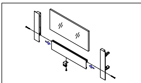
Drawer Front assembly
