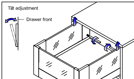
Tilting adjustment
