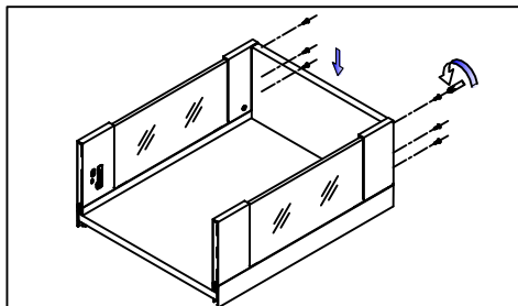
Back assembly
