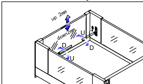
Up / down adjustment
