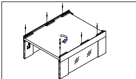
Bottom assembly
