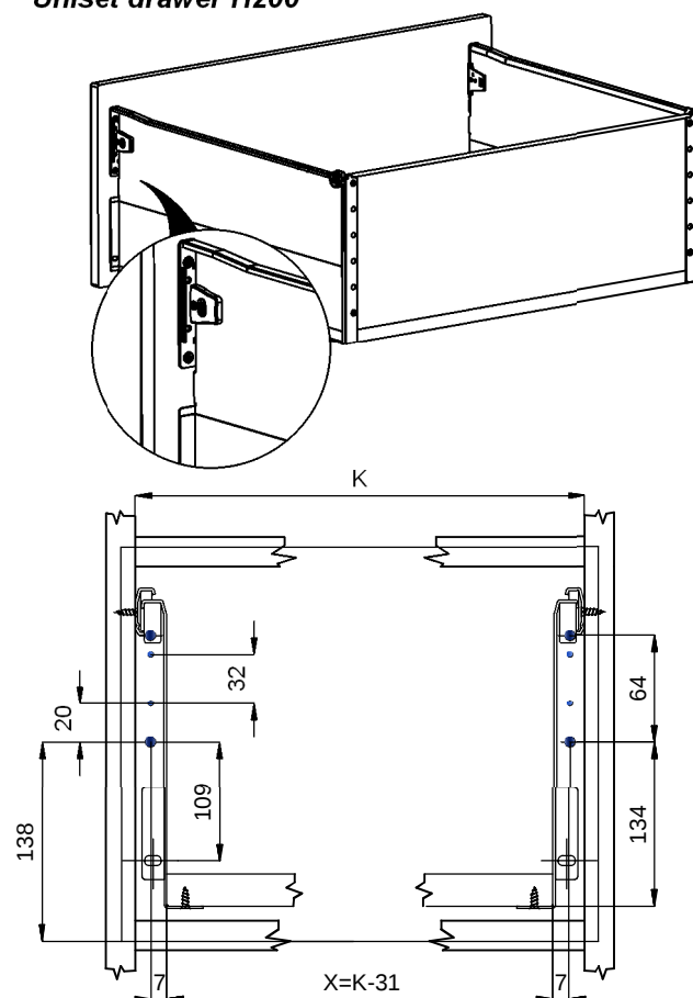
Tiroir Uniset H200 Uniset drawer H200
