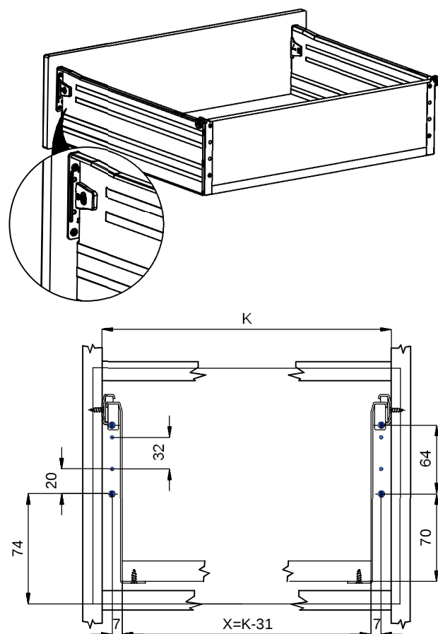
Tiroir Uniset H150 Uniset drawer H150
