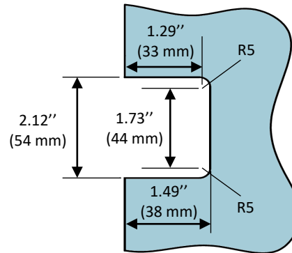
Glass Strike Cut-out
